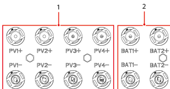
Figura 5-11 Bornes
